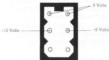
Diagram B Looking INTO power connector on 'BBC' compatible drives.
